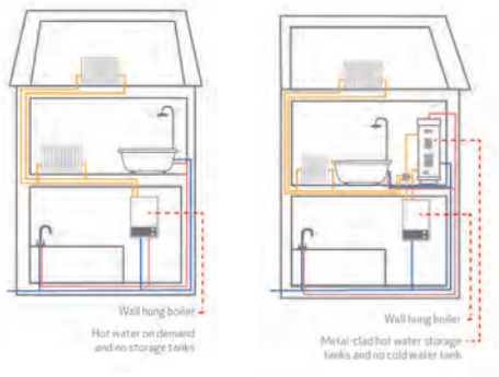
Mains-fed: combination boiler Mains-fed: unvented cylinder
