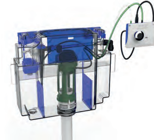
Vantage Electroflo Infrared Dual Flush Cistern
