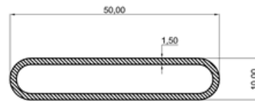
Sec. B-B
